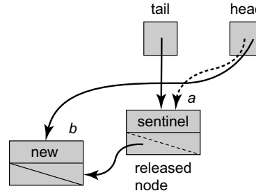
Figure 10.13 Why dequeuers must help advance tail in Line 35 of Fig. 10.11. Consider the scenario in which a thread enqueueing node b has redirected a 's next field to b , but has yet to redirect tail from a to b . If another thread starts dequeuing, it will read b 's value and redirect head from a to b , effectively removing a while tail still refers to it. To avoid this problem, the dequeuing thread must help advance tail from a to b before redirecting head .
