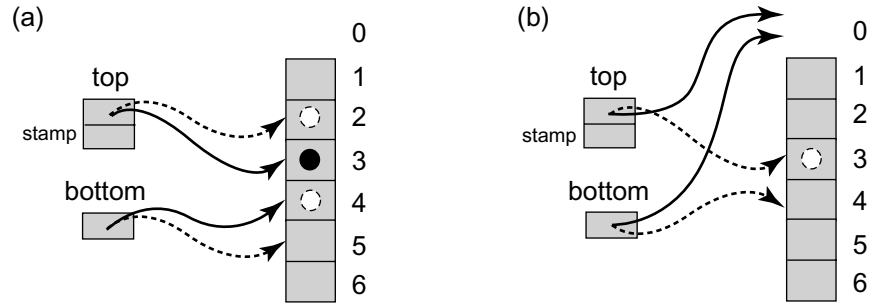
Figure 16.12 The BoundedDeque implementation. In Part (a) popTop() and popBottom() are called concurrently while there is more than one task in the BoundedDeque. The popTop() method reads the element in entry 2 and calls compareAndSet() to redirect the top reference to entry 3. The popBottom() method redirects the bottom reference from 5 to 4 using a simple store and then, after checking that bottom is greater than top it removes the task in entry 4. In Part (b) there is only a single task. When popBottom() detects that after redirecting from 4 to 3 top and bottom are equal, it attempts to redirect top with a compareAndSet() . Before doing so it redirects bottom to 0 because this last task will be removed by one of the two popping methods. If popTop() detects that top and bottom are equal it gives up, and otherwise it tries to advance top using compareAndSet() . If both methods apply compareAndSet() to the top , one wins and removes the task. In any case, win or lose, popBottom() resets top to 0 since the BoundedDeque is empty.
