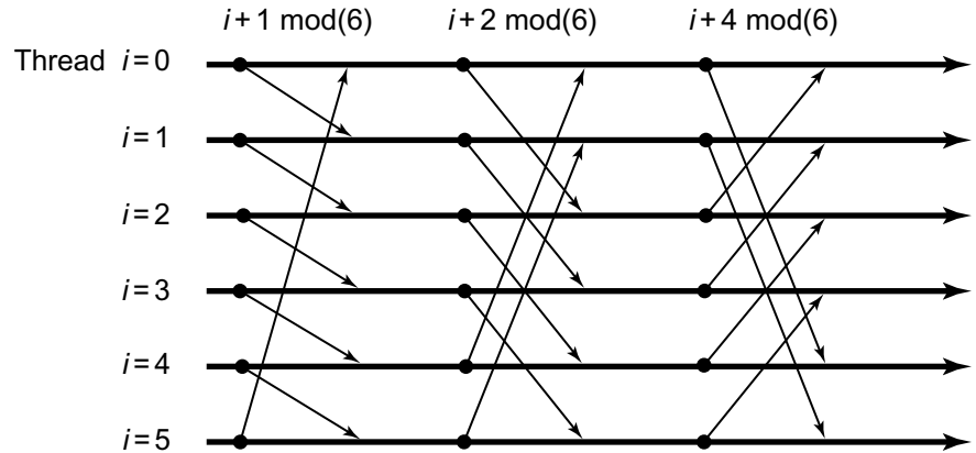
Figure 17.21 Communication in the dissemination barrier. In each round r a thread i communicates with thread i+2^r(\bmod n) .
