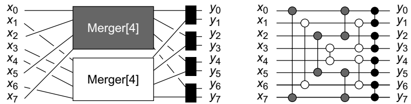
Figure 12.12 On the left-hand side we see the logical structure of a MERGER [8] network, into which feed two BITONIC [4] networks, as depicted in Fig. 12.12. The gray MERGER [4] network has as inputs the odd wires coming out of the top BITONIC [4] network, and the even ones from the lower BITONIC [4] network. In the lower MERGER [4] the situation is reversed. Once the wires exit the two MERGER [4] networks, each pair of identically numbered wires is combined by a balancer. On the right-hand side we see the physical layout of a MERGER [8] network. The different balancers are color coded to match the logical structure in the left-hand figure.
