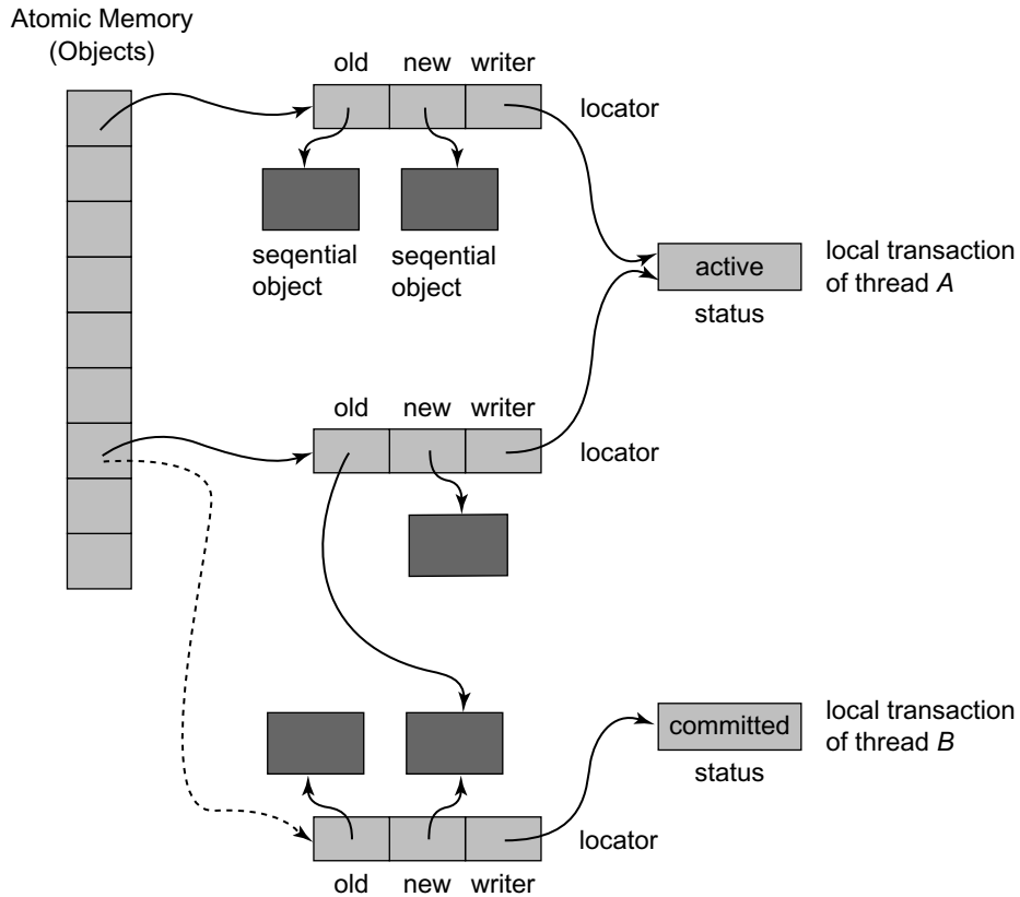
Figure 18.21 The FreeObject class: an obstruction-free atomic object implementation. Thread A has completed the writing of one object and is in the process of switching a copy of the a second object that was last written by thread B. It prepares a new locator with a fresh new copy of the object and an old object field that refers to the new field of thread B's locator. It then uses a compareAndSet() to switch the object to refer to the newly created locator.
