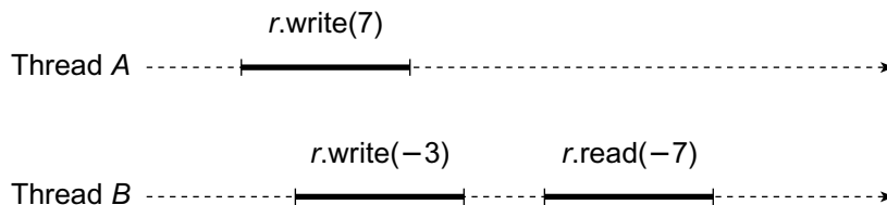
Figure 3.4 Why each method call should appear to take effect instantaneously. Two threads concurrently write -3 and 7 to a shared register r . Later, one thread reads r and returns the value -7 . We expect to find either 7 or -3 in the register; not a mixture of both.
