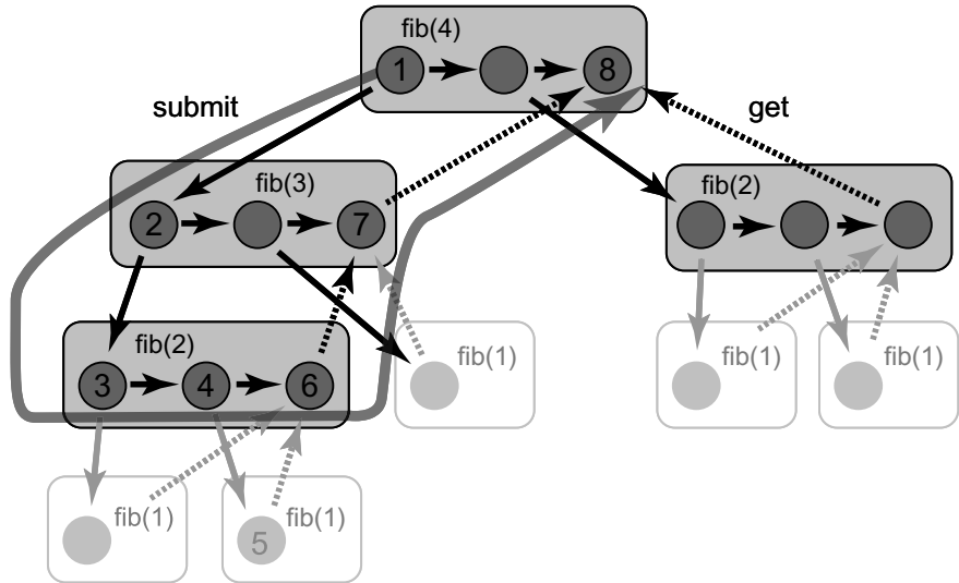
Figure 16.8 A sub-DAG in the 6th step of the FibTask(4) computation. The grey line marks the longest path. We know that the last step of FibTask(2), which is next on the critical path, is ready to execute because the steps it depends on have been completed (it has no incoming edges apart from its preceding step in program order). Moreover, we know this is an idle step: there is not enough work for all the processors. But the scheduler is greedy, so we must have scheduled the last step of FibTask(2) in this step. This is an example of how every idle round shortens this critical path by one node (other steps may shorten it too, but we do not count them).
