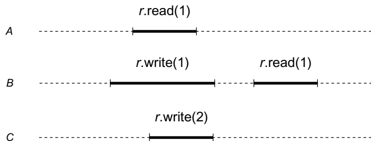
Figure 3.14 Second history for Exercise 24.
