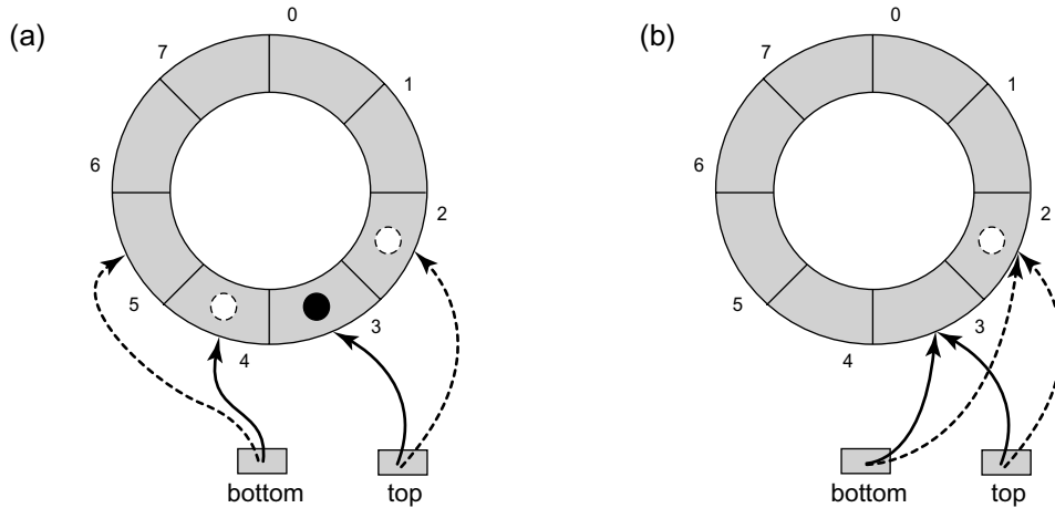
Figure 16.16 The UnboundedDeque class implementation. In Part (a) popTop() and popBottom() are executed concurrently while there is more than one task in the UnboundedDeque object. In Part (b) there is only a single task, and initially bottom refers to Entry 3 and top to 2. The popBottom() method first decrements bottom from 3 to 2 (we denote this change by a dashed line pointing to Entry 2 since it will change again soon). Then, when popBottom() detects that the gap between the newly-set bottom and top is 0, it attempts to increment top by 1 (rather than reset it to 0 as in the BoundedDeque). The popTop() method attempts to do the same. The top field is incremented by one of them, and the winner takes the last task. Finally, the popBottom() method sets bottom back to Entry 3, which is equal to top .
