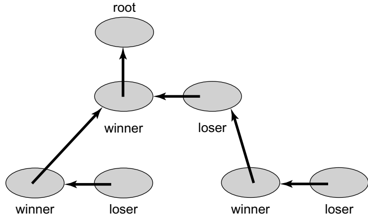
Figure 17.17 The TourBarrier class: information flow. Nodes are paired statically in active/passive pairs. Threads start at the leaves. Each thread in an active node waits for its passive partner to show up; then it proceeds up the tree. Each passive thread waits for its active partner for notification of completion. Once an active thread reaches the root, all threads have arrived, and notifications flow down the tree in the reverse order.
